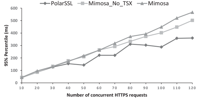
Figure 5: 95% Percentile Latencies of HTTPS
