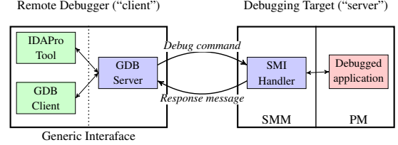
Fig. 3. Using MALT with Multiple Debugging Clients
