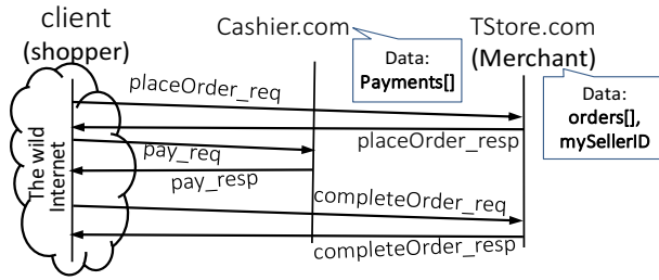
Figure 3: The basic messages and data for checkout.
