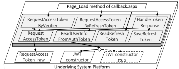
Figure 11: Factoring and stubbing in callback.aspx.
