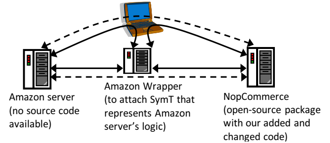
Figure 12: An example wrapper service.
