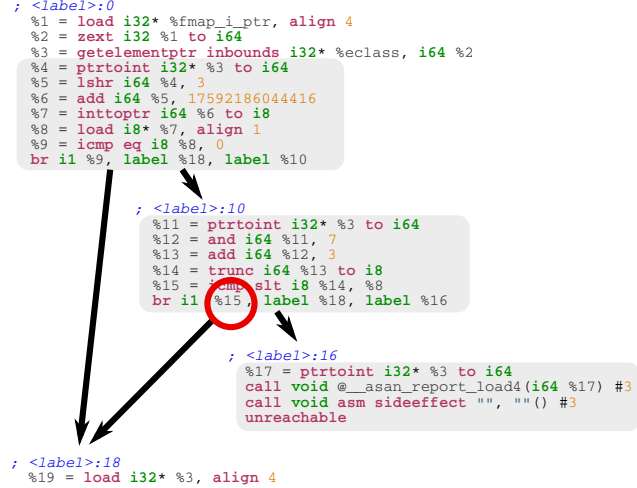
Fig. 4. A sanity check inserted by AddressSanitizer, in the LLVM intermediate language. The corresponding C code is cc1 = ec1ass[fmap[i]] and is found in blocksort.c in the bzip2 SPEC benchmark. Instructions belonging to the check are shaded. The red circle marks the branch condition which, when set to true , will cause the check to be eliminated.
